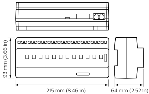
Dynalite Relay Controllers
