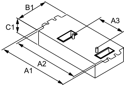
ELE DIM BALLAST (2) 18W CFL (4-PIN) 120V
