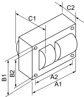
HPS BAL 250W S50 5-TAP KIT WITH LAMP
