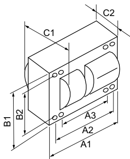
MH BAL 1500W M48 220V C&C
