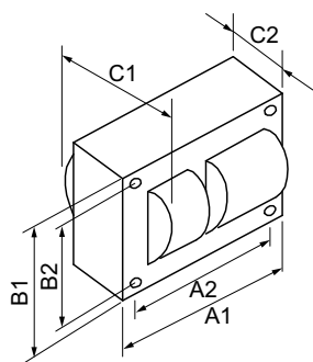
HPS BAL 250W S50 5-TAP C&C
