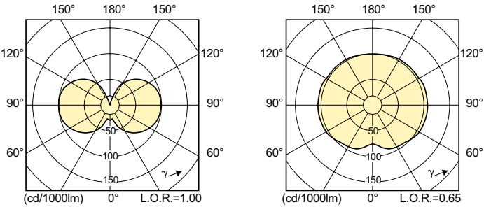
Light Distribution Diagram - MASTERC CDM-TM MINI 35W/930 PGJ5 KIT/12
