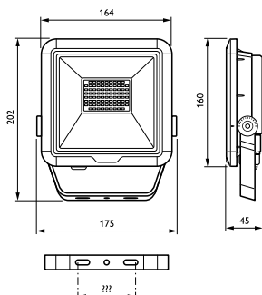
PA2-LED Outdoor
