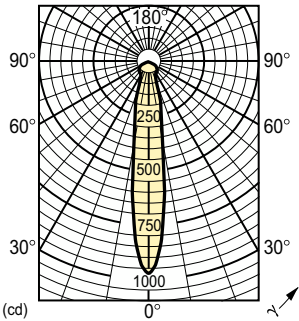
Light Distribution Diagram - Refl 60W E27 230V NR80 25D 1CT/30
