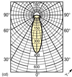
Light Distribution Diagram - Refl 40W E14 240V NR50 30D 1CT/30
