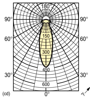
Light Distribution Diagram - Refl 40W E14 240V NR50 30D FR 2BC/10
