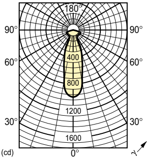
Light Distribution Diagram - SPOT 60W E27 220-240V NR63 30D FR 1CT
