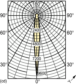
Light Distribution Diagram - PAR38 120W E27/51 115V Spot 1CT/15
