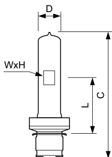
6996C 1000W P28s 240V
