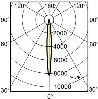
Light Distribution Diagram – Brill 35W GU4 12V 10D 1CT/10X5F
