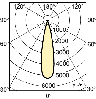
Light Distribution Diagram - MASTERLine 111 45W G53 12V 24D 1CT/6
