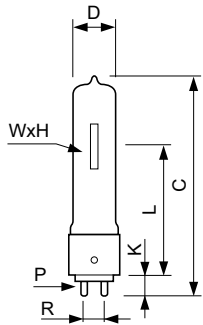
6983P 1000W G9.5 230V
