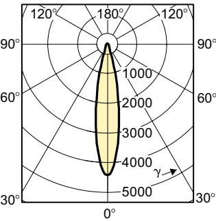
Light Distribution Diagram - MASTERL ES 35W GU5.3 12V 24D 1CT/4X5F
