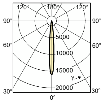
Light Distribution Diagram - MASTERL ES 45W GU5.3 12V 8D 1CT/4X5F
