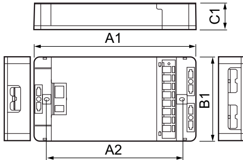
Lumiblade Driver D230V 80W/0.1-0.5A/28V
