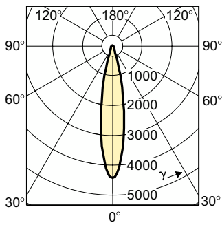
Light Distribution Diagram - EnAdvIR Alu 35W 12V MR16 24D 1CT/4XF5
