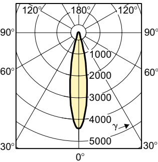
Light Distribution Diagram - EnAdvIR Alu 35W 12V MR16 24D 1CT/4XF5
