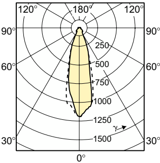
Light Distribution Diagram - BC50 TWISTLINE GU10/FL25 12CT/6
