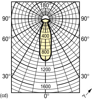
Light Distribution Diagram - Refl 60W E27 230V NR63 30D FR 1CT/30
