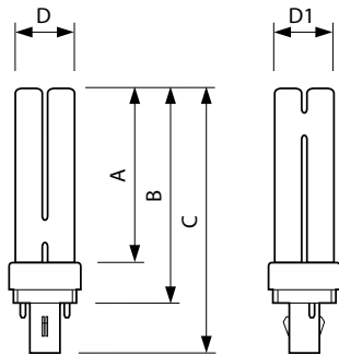
28W/827 GX32d-3 PL-C ES
