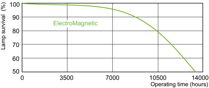
Life Expectancy Diagram - PL-S 5W/841/2P/ALTO
