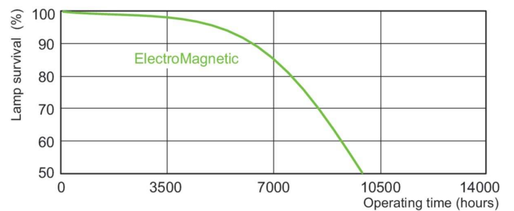
Life Expectancy Diagram - PL-S 7W/835/2P/ALTO
