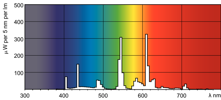
Spectral Power Distribution Colour - PL-S 7W/835/2P/ALTO
