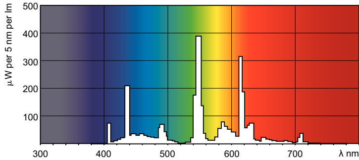
Spectral Power Distribution Colour - MASTER PL-L 24W/840/4P UNP/50
