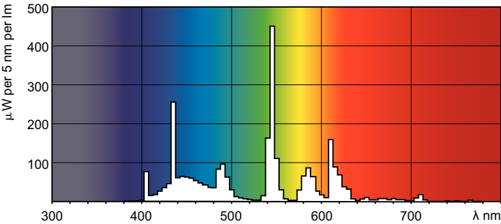
Spectral Power Distribution Colour - MASTER PL-C 10W/865/2P 1CT/5X10BOX
