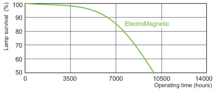
Life Expectancy Diagram - MASTER PL-C 10W/865 1CT/5X10CC
