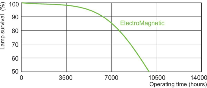
Life Expectancy Diagram - MASTER PL-C 13W/827/2P 1CT/5X10BOX
