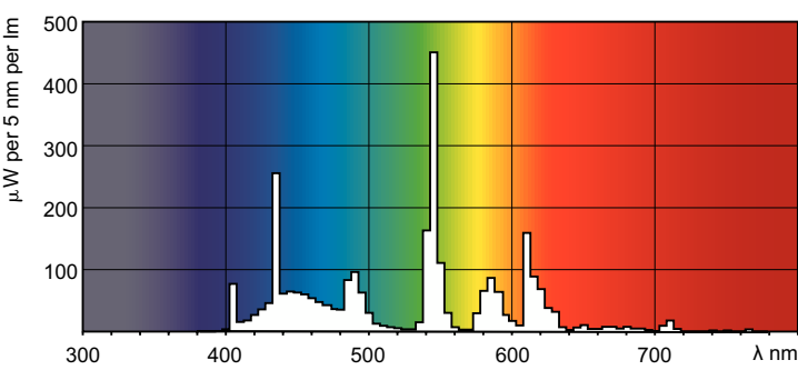
Spectral Power Distribution Colour - MASTER PL-C 13W/865/2P 1CT/5X10BOX
