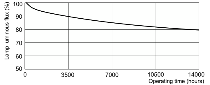
Lumen Maintenance Diagram - MASTER PL-C 18W/830/2P 1CT/5X10BOX
