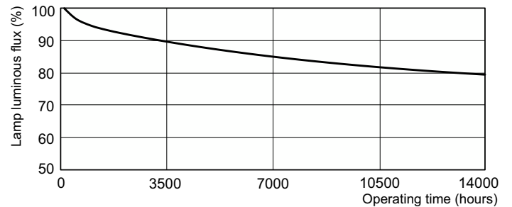
Lumen Maintenance Diagram - MASTER PL-C 26W/827/2P 1CT/5X10BOX
