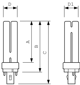
PL-C 26W/840/2P
