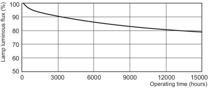
Lumen Maintenance Diagram - MASTER PL-C 10W/830/4P 1CT/5X10BOX
