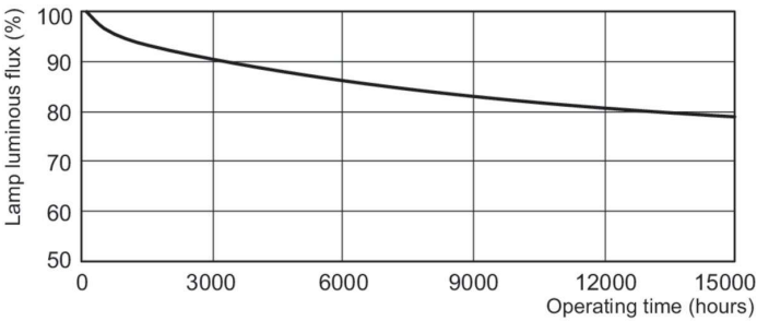
Lumen Maintenance Diagram - MASTER PL-C 10W/840/4P 1CT/5X10BOX
