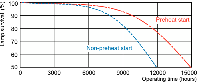
Life Expectancy Diagram - PL-C 13W/835/4P/ALTO 10PK
