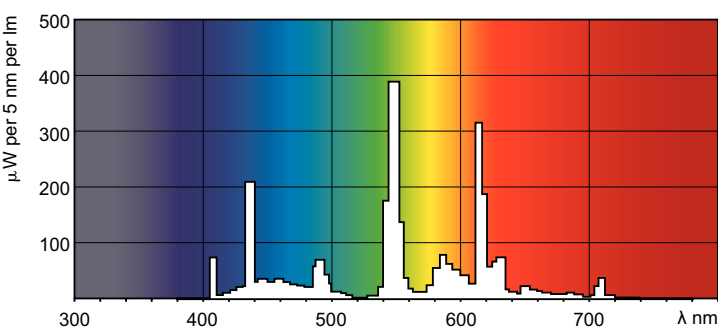
Spectral Power Distribution Colour - MASTER PL-C 13W/840/4P 1CT/5X10BOX
