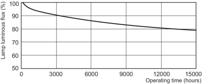
Lumen Maintenance Diagram - MASTER PL-C 13W/865/4P 1CT/5X10BOX
