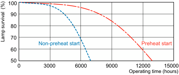
Life Expectancy Diagram - MASTER PL-C 18W/830/4P 1CT/5X10CC
