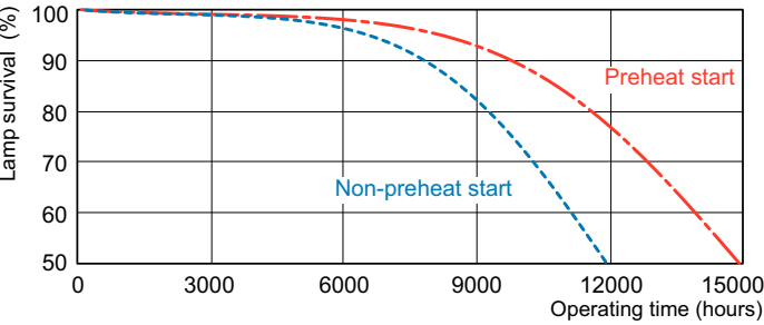
Life Expectancy Diagram - MASTER PL-C 18W/830/4P 1CT/5X10CC
