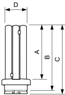
PL-R 14W/830/4P
