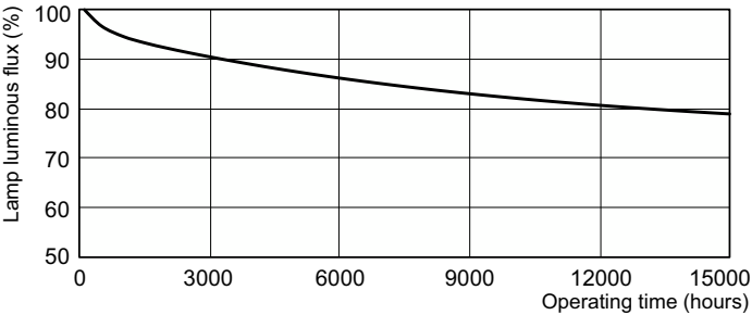
Lumen Maintenance Diagram - PL-T 26W/841/A/4P 1CT/5X10BOX ALTO
