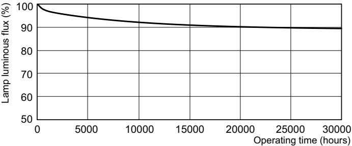
Lumen Maintenance Diagram - MASTER TL-D Super 80 15W/827 SLV/25
