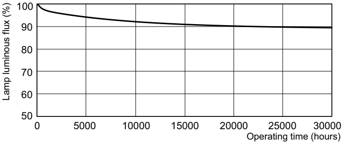
Lumen Maintenance Diagram - MASTER TL-D Super 80 15W/840 SLV/25
