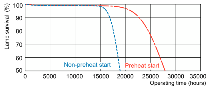
Life Expectancy Diagram - TL5 HE 14W WW 1PP/10
