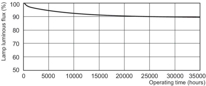
Lumen Maintenance Diagram - MASTER TL5 HE 21W/840 SLV/20
