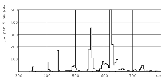
Lightcolour /827
