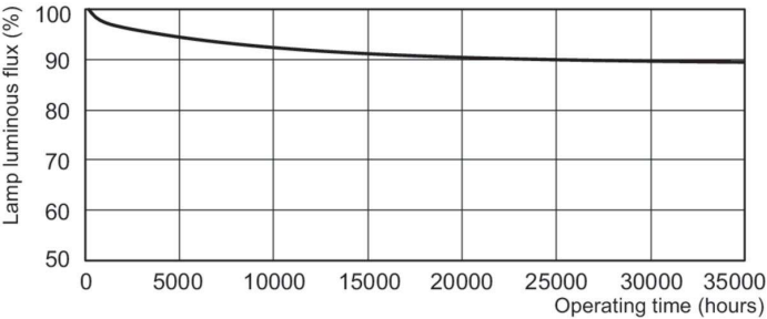
Lumen Maintenance Diagram - MASTER TL5 HE 35W/840 SLV/40
