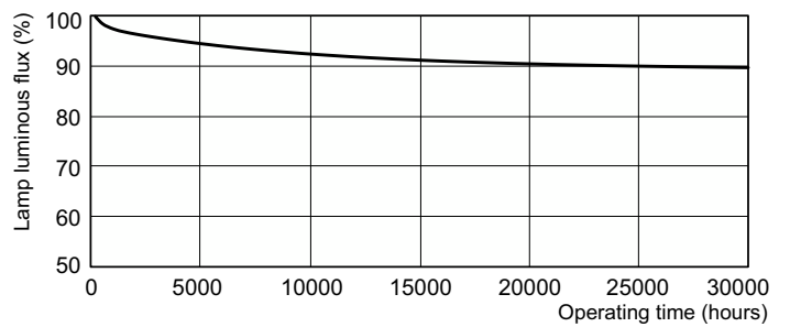
Lumen Maintenance Diagram - MASTER TL5 HO 39W/865 SLV/40
