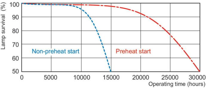
Life Expectancy Diagram - MST TL5 HO ActiViva Active 54W 1SL/40
