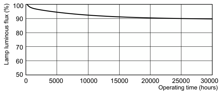
Lumen Maintenance Diagram - MST TL5 HO ActiViva Active 54W 1SL/40
